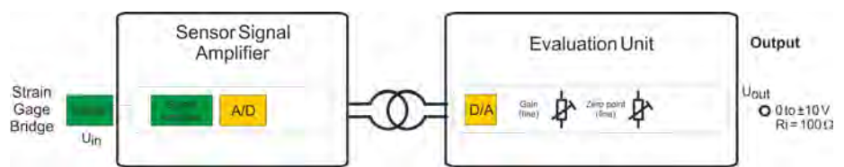
Fig. 2: Block diagram
