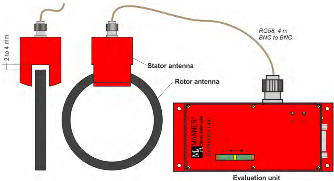
Fig. 5: Coupling
