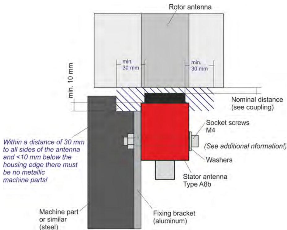
Fig. 6: Minimum distance antenna A8b
