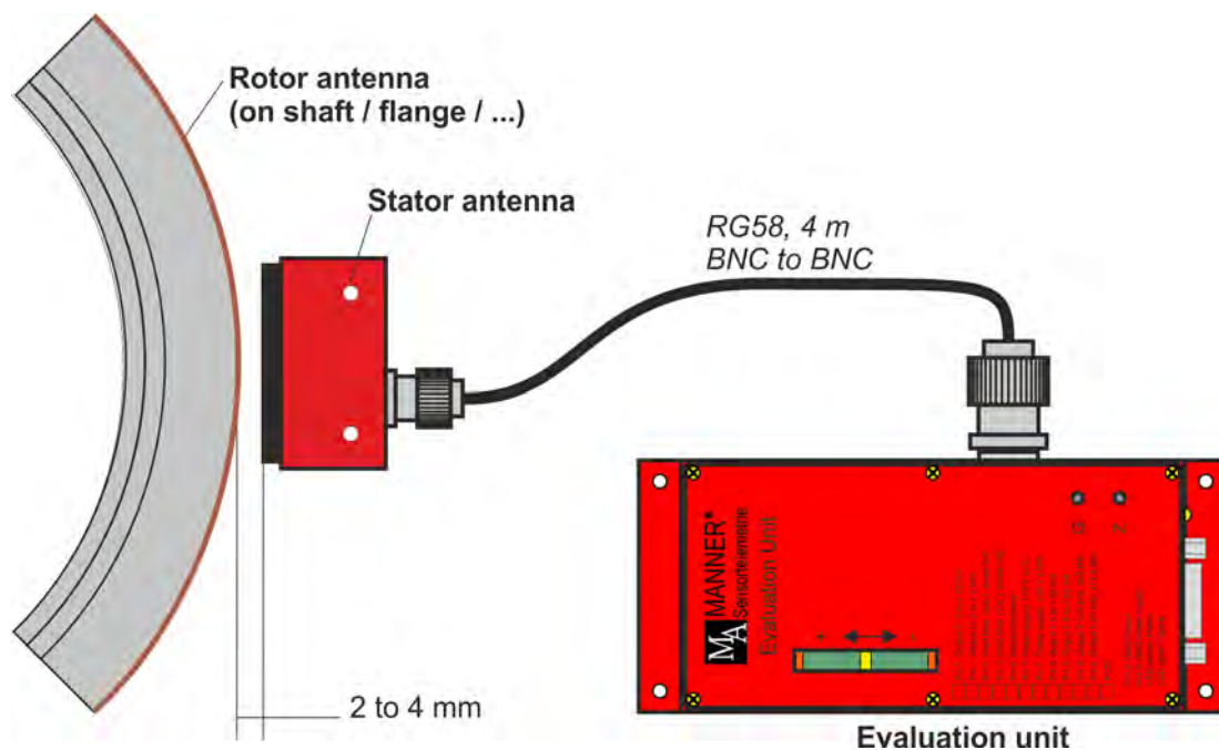
Fig. 5: Coupling
